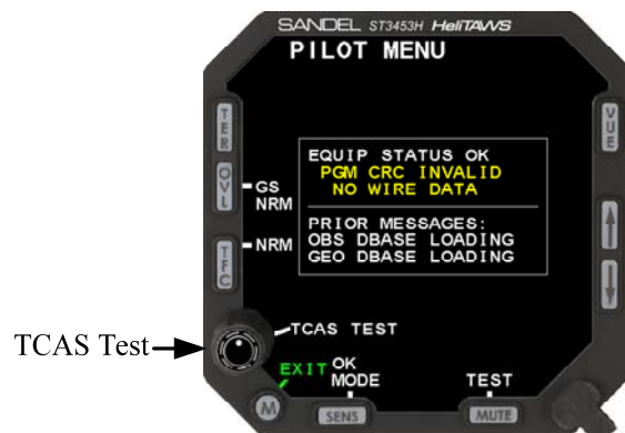
Figure 10-4 TCAS Test
