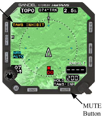
Figure 7-5 TAWS INHIBIT
