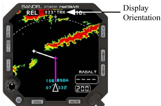
Figure 5-11 Display Orientation
