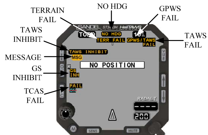
Figure 12-1 On-Screen Annunciation
