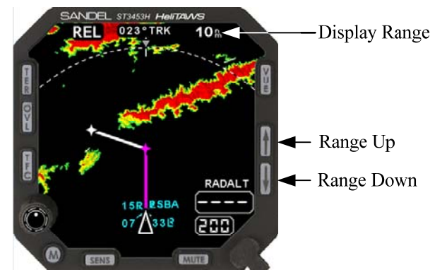
Figure 5-12 Display Ranging
