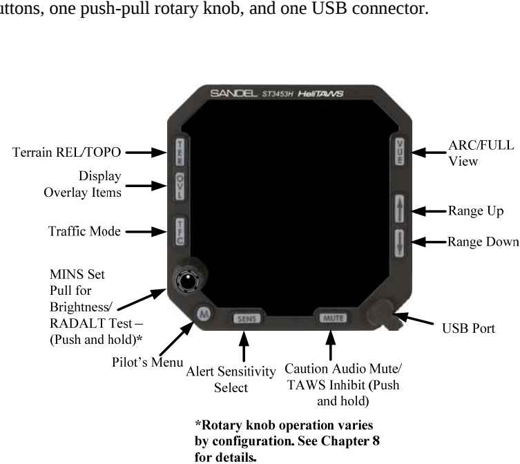
Figure 5-1 ST3453H Physical Features
