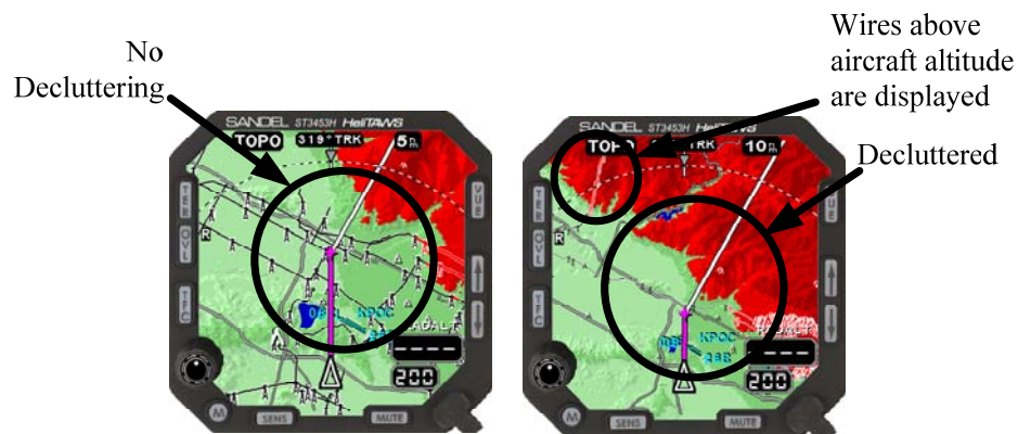
Figure 5-13 Decluttering
