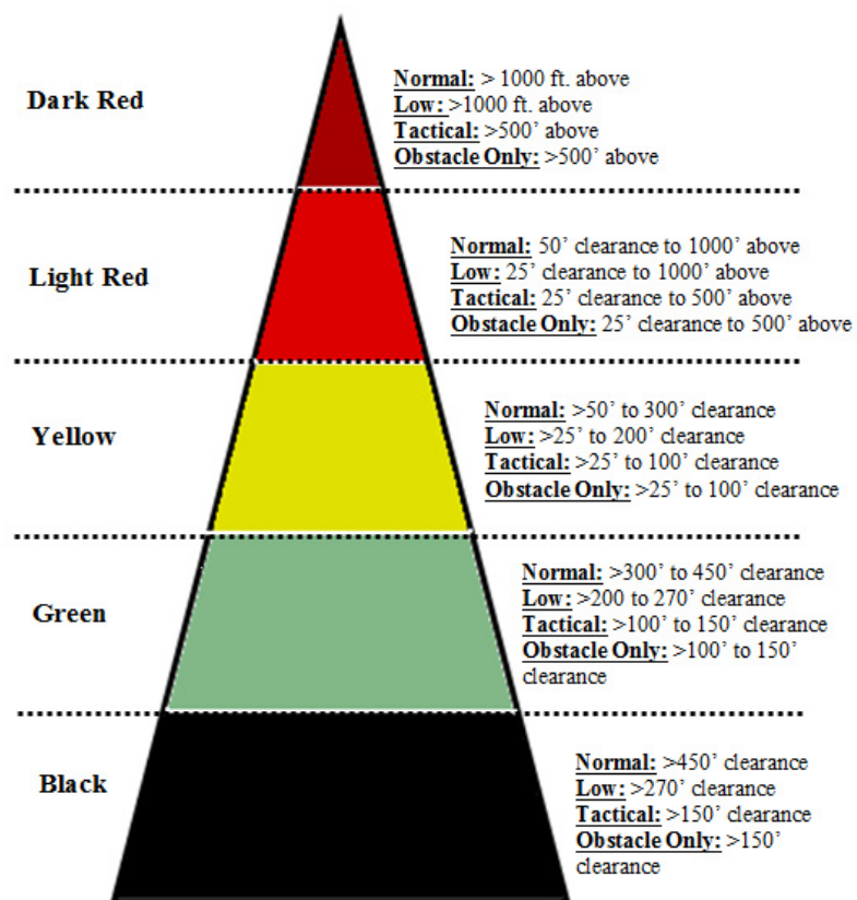
Figure 5-10 REL Display Color Banding Relative to Aircraft Altitude
