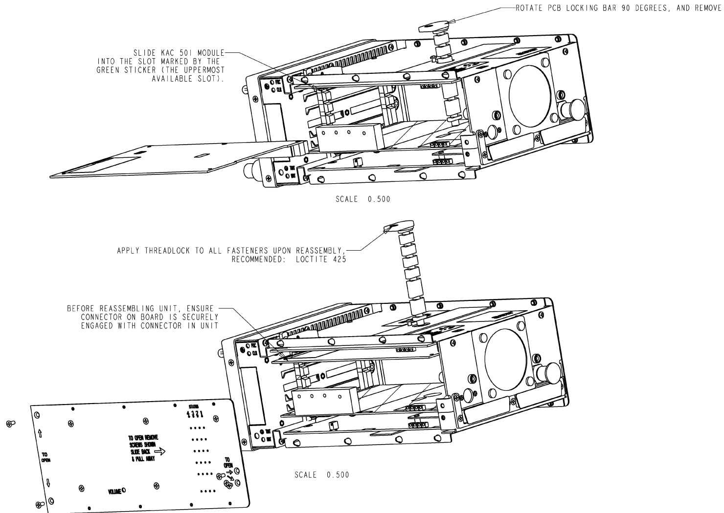
Figure 2-5 KAC 501 INSTALLATION DRAWING (P/N 155-01737-0000 Rev. A, Sheet 2 of 2)
