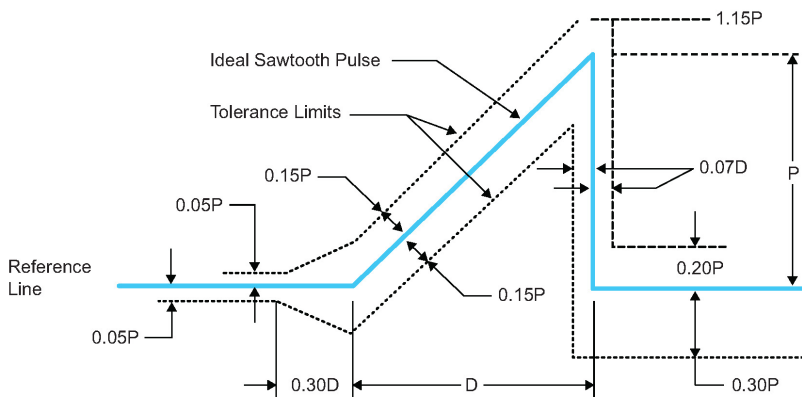
Figure 3-1. Peak Shock Levels
